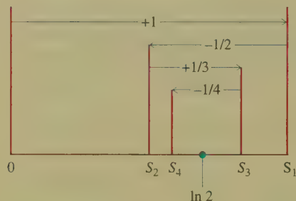
Figure 10.9 The partial sums of this alternating series oscillate back and forth on either side of their eventual sum, \ln 2 . This guarantees that the truncation error is always less than the first omitted term of the series in magnitude.
